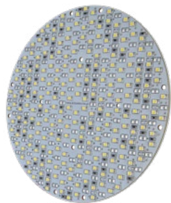
OPEN TYPE LED BOARD Ø155mm
